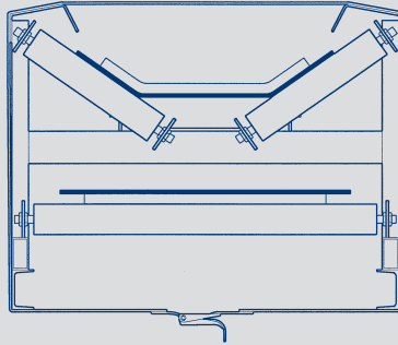
Standard Boom Section Suitable for machines up to 24 metres boom length and belt widths to 1000 mm as shown below
