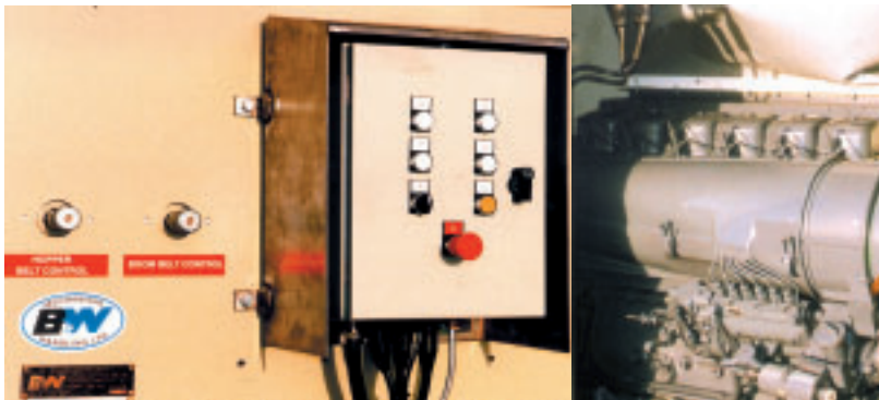
External control panel for diesel motor drive showing local engine key switch starting control without full instrumentation
