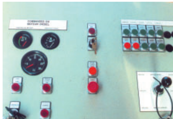
Comprehensive control panel with integral diesel motor instrumentation and joy stick controller for powered travel system operation
