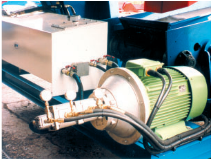
Electric Motor Drive with direct coupled triple section hydraulic pump and reservoir mounted beneath the Samson® section
