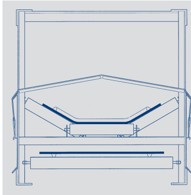
Tapered Boom Section Suitable for machines over 24 metres boom length and belt widths to 1200 mm
