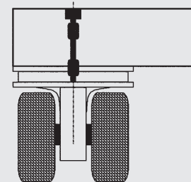
Rotary Potentiometer linked to the steering system provides automated wheel alignment in any travel mode
